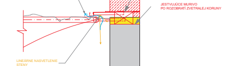
DETAIL "A"
