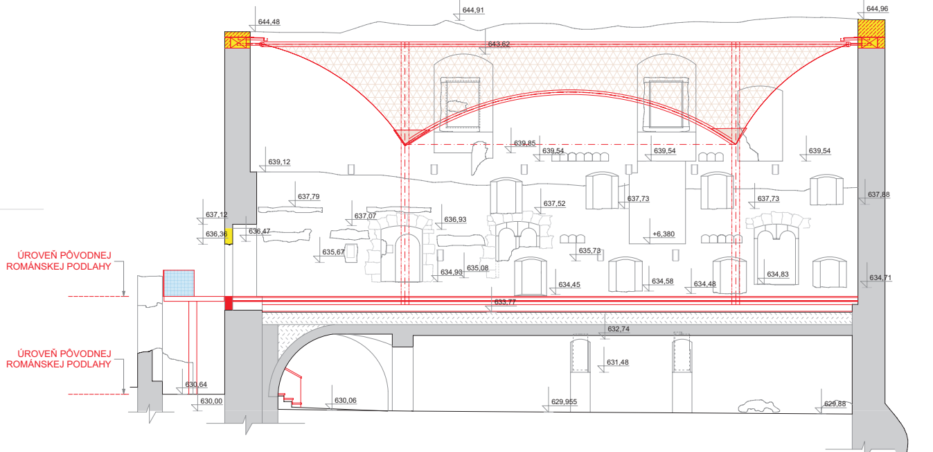
DETAIL "A"
